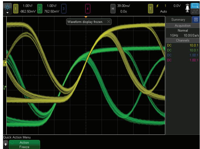
Figure 57. Quick Freeze Display preserves the persistence.
